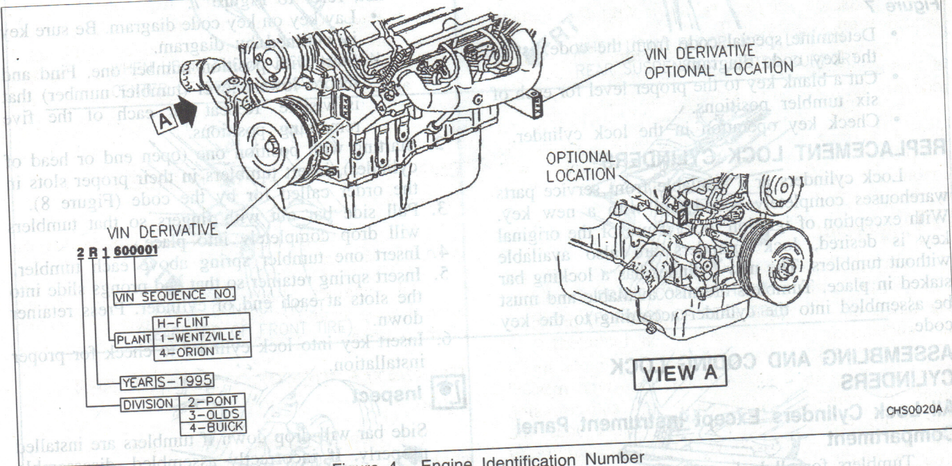
Figure 4 - Engine Identification Number
